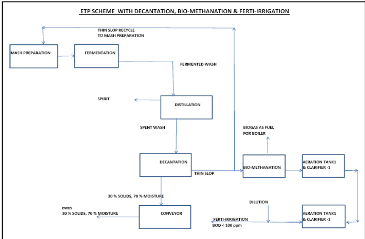
Existing Plant scheme of the ETP
